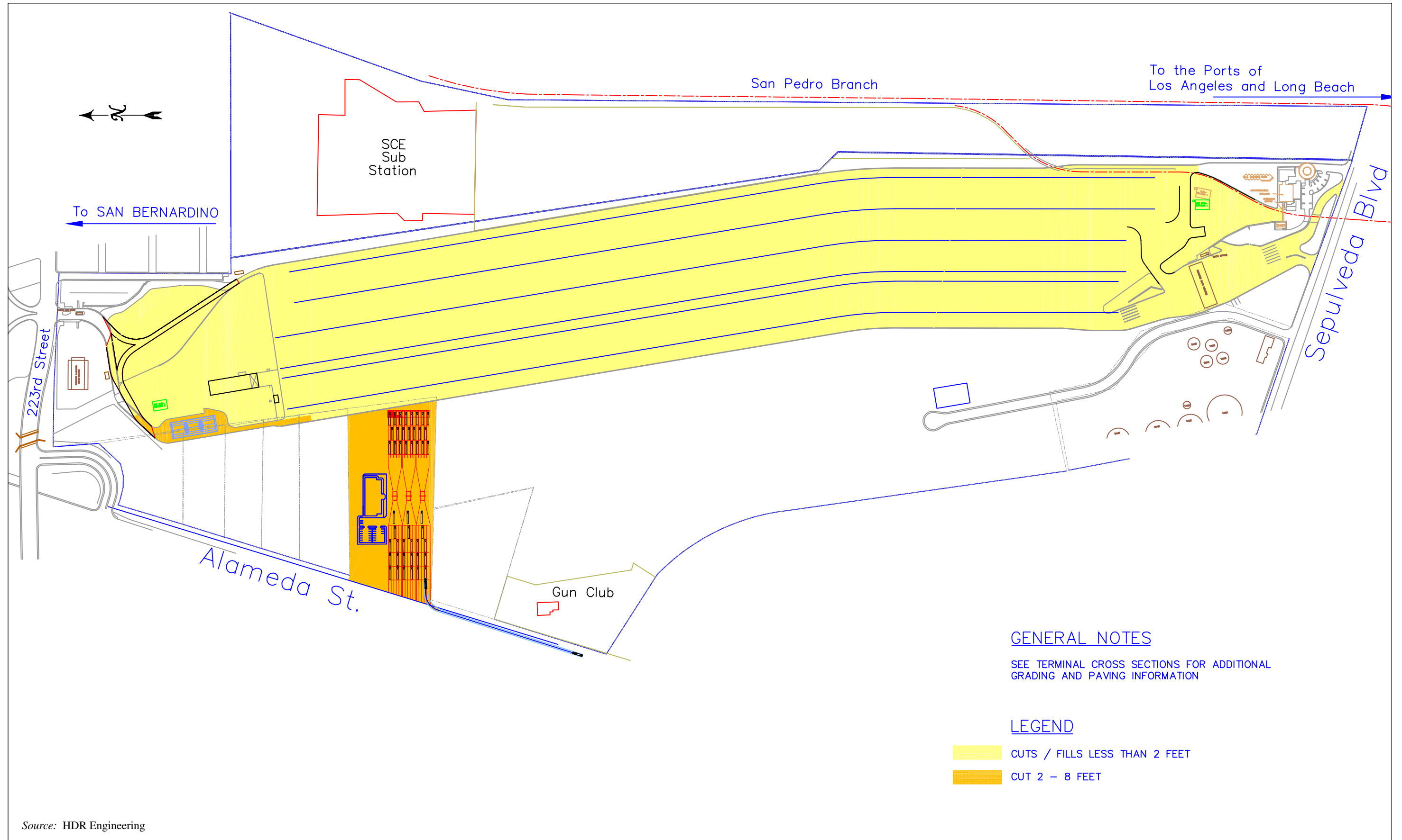
Figure 11. UP ICTF Conceptual Grading Plan
